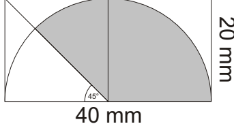
Feed cone cutout
